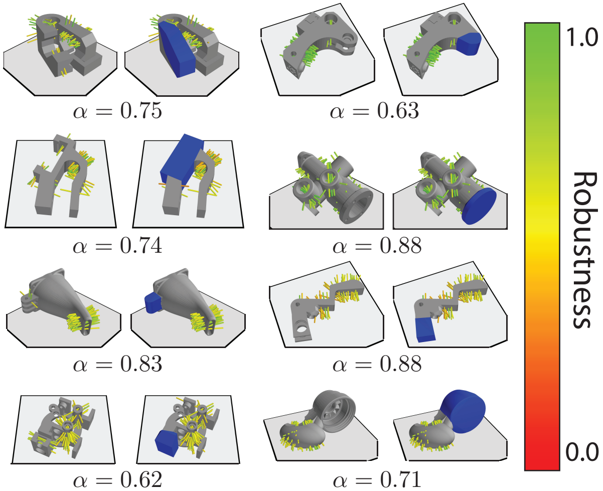
Fig. 7: For eight parts, a comparison of the top 50 most robust grasps from the executable grasp set on the original part (left) and planned our algorithm using convex hull masking (right). The coverage \alpha is reported for each of our computed privacy-preserving grasp sets, and proprietary zones are marked in blue. Each grasp axis is colored by its robustness, or probability of force closure ( P_F ) under uncertainty in object pose, gripper pose, and friction. Grasp sets planned by our algorithm are similar to those planned without considering privacy, and that the computed sets do not intersect the private region of the original mesh, suggesting that grasps planned on the masked part preserve privacy and cover the public region of the original part, and that robust grasps tend to be clustered on certain areas of the part.
