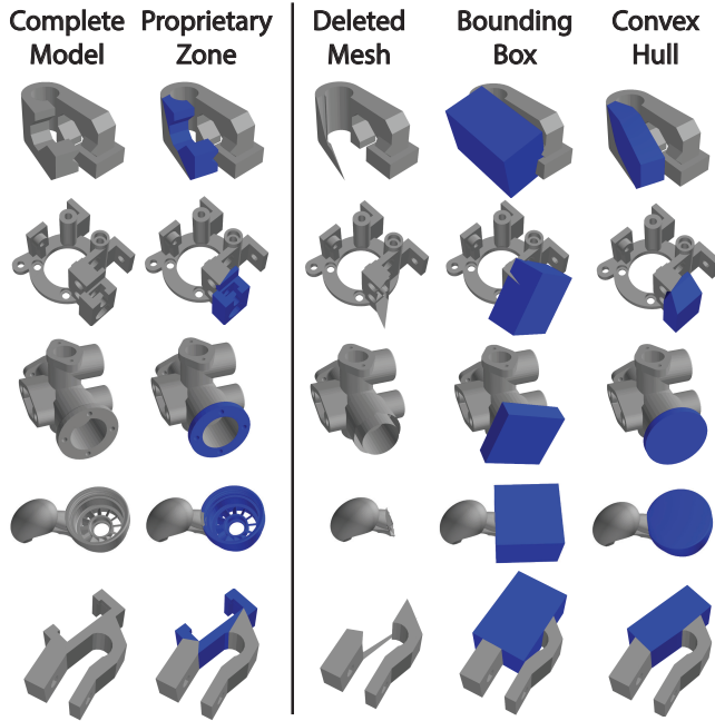
Fig. 4: Illustration of the different methods for masking proprietary zones (highlighted in blue) on five example parts. (Left to right) One method to mask parts is to delete the proprietary zone of the mesh, however this can lead to planned grasps in collision on the original object. To avoid collisions, the proprietary zone can be replaced with its bounding box or convex hull.
