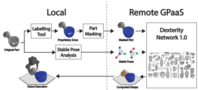
Fig. 1: Overview of privacy-preserving grasp planning. Industrial users label proprietary zones on the part with a graphical interface. The masked object is then transmitted to a Cloud-based grasp planner along with its stable poses. The grasp planner computes a set of grasps for each stable pose and returns the grasp sets to the user.
