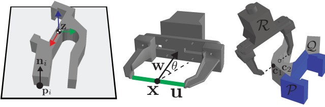
Fig. 2: Illustration of our notation. (Left) The object frame of reference is centered at the center-of-mass \mathbf{z} . Each object is associated with a set of stable poses (planar worksurface orientations) defined by the plane (\mathbf{n}_i, \mathbf{p}_i) . (Middle) We can parameterize parallel-jaw grasps by their center \mathbf{x} and axis \mathbf{u} , which defines a gripper pose when the angle \theta of the gripper approach axis \mathbf{w} is specified. (Right) A parallel-jaw gripper \mathcal{R} contacts a mesh \mathcal{M} at points \mathbf{c}_1 and \mathbf{c}_2 . The space of all possible grasps is the space of all contact pairs. Each mesh is divided into a private region \mathcal{P} (blue) and public region \mathcal{Q} (grey).
