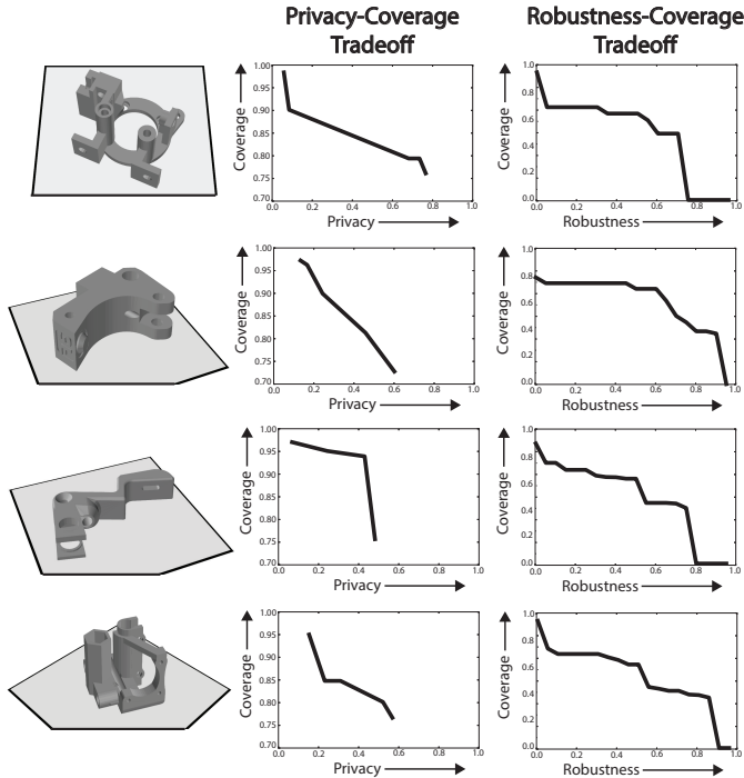
Fig. 6: Plotting the privacy-coverage tradeoff and robustness-coverage tradeoff for four example parts (a gearbox, an extruder, a nozzle mount, and an idler mount), each with a sequence of nested proprietary regions. The functions are monotone but nonlinear because the set of robust grasps may be more dense in particular regions of the mesh, and jumps occur when areas of high density are masked.
