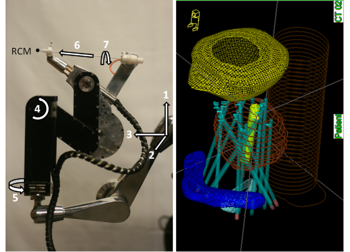
Fig. 1. The left figures shows 7-DoF Acubot-RND robot: a 3-DoF cartesian stage (1,2 and 3), a rotating center of motion (4 and 5), needle insertion and needle rotation (6 and 7). The right figure shows a skew-Line needle arrangement implanted by the semi-autonomous robot assisted system. The figure is obtained after CT-Scanning of tissue phantom, and contouring the structures in the digital form.
