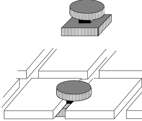
Figure 6: T-slot fixels are equivalent to clamps in our model.
