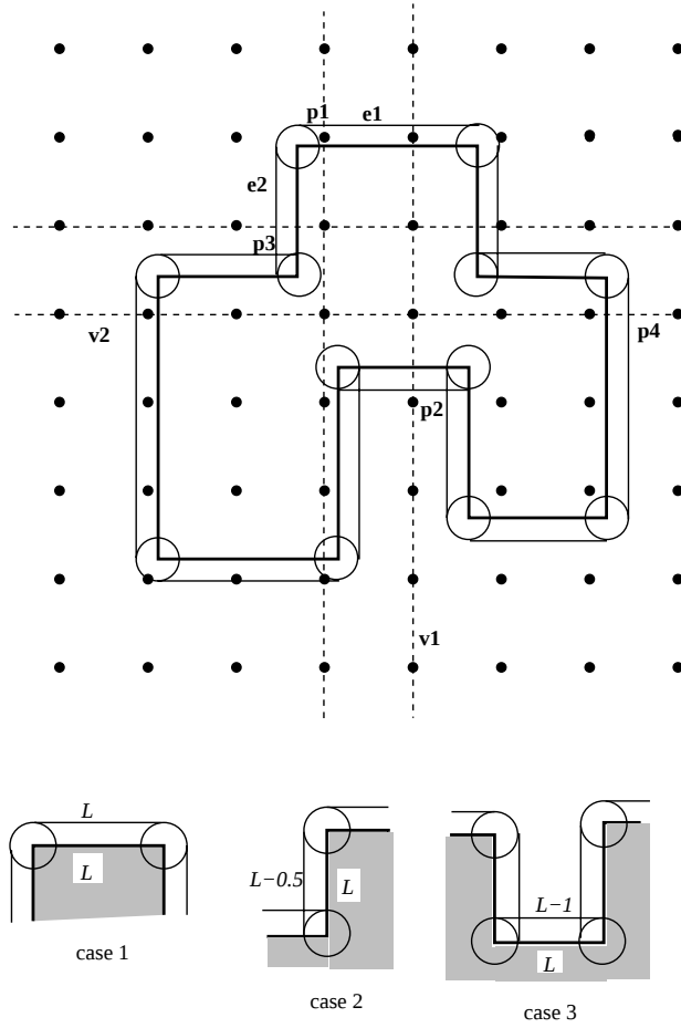
Figure 8: The expanded rectilinear part. At the top, a grown part that can be fixtured by point fixels. At the bottom, three cases of the straight edges in the grown rectilinear part, where the shadow stands for the interior of a part. All variables are corresponding to the proof of Theorem 4.
