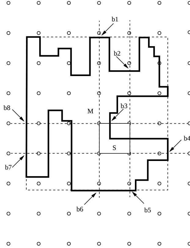
Figure 7: A rectilinear part and possible clamp positions: all variables correspond to the proof of Theorem 2.
