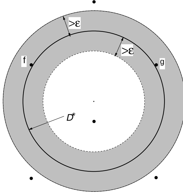
Figure 5: Intuition behind the proof: All lattice sites except f and g are outside an annulus of width 2\epsilon , where D^* is the disk constructed by lemma 1. Thus the polygon cannot be shifted to make contact with a third lattice site without losing contact with f and g .
