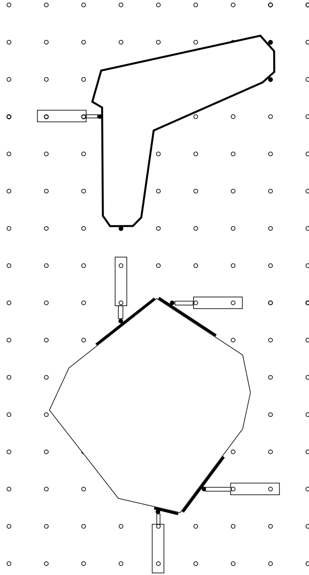
Figure 1: Examples of parts in modular fixtures. At top, a part fixtured with 3 locators and one clamp. At bottom, a part fixtured using 4 clamps.
