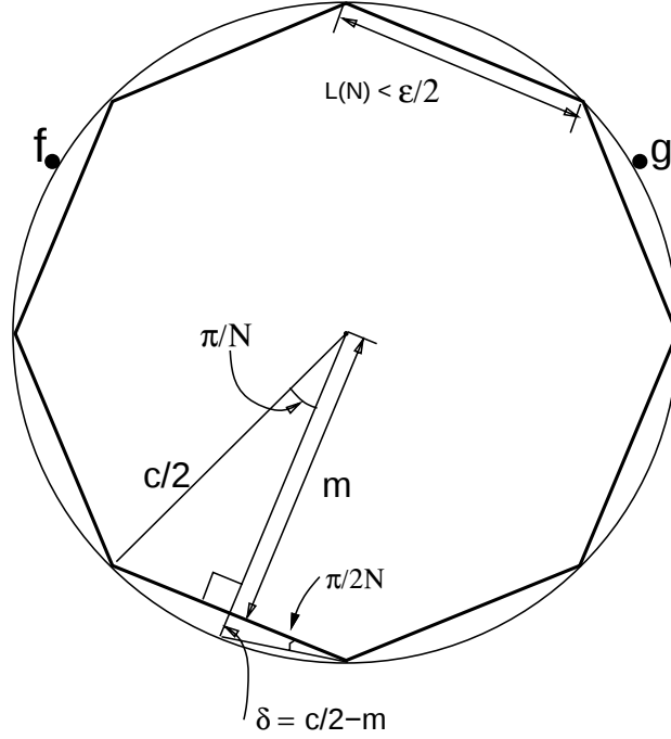
Figure 4: Illustration of how to transform the disk into an unfixturable polygon: all variables are as in the proof of the Theorem 1.
