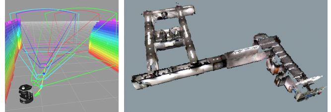
(a) Mapping an indoor environment with a ground robot
