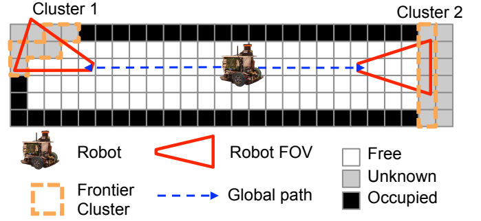
Fig. 5: Global Planning: We generate global plans by 1) clustering frontier voxels and 2) planning paths to destinations that can view them. When a robot can view a cluster from multiple places, we select the one that can be reached the fastest.
