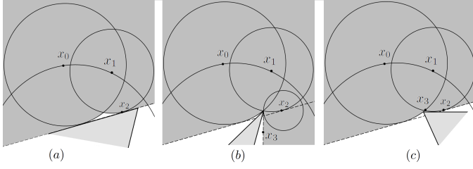
Fig. 7. The third probe from x_2 results in the disk C_2 . There are three possible cases: (a) If C_2 is a zero disk, then three probes are sufficient to confirm the first edge. (b) If \partial(C_2) intersects the intersection of \partial(C_0), \partial(C_1) , the intersection point is confirmed as a vertex and probing from x_3 will be tangent to the adjacent edge. (c) Otherwise, probing from x_3 (the intersection point of \partial(C_0), \partial(C_1) ) will confirm an edge and one of its endpoints.
