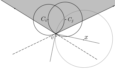
Fig. 3. If v is a confirmed vertex and the disk resulting from x \in R is tangent to v , then \angle_P(v) is acute while \angle_R(v) is not acute.
