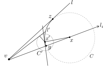
Fig. 4. The ray l' with source at v and tangent to C' cannot be tangent to C' inside of C , where C' is a disk centered at an arbitrary point lying on \partial(C) and between y and z .
