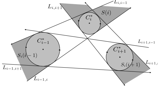
Fig. 2. An example of three consecutive cp-disks, which shows the shadow sets of C_{i-1}^* , C_{i+1}^* with respect to C_i^* and the neighbor-shadow set of C_i^* .
