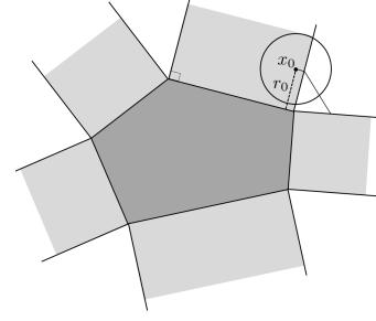
Fig. 6. The partitioning of the exterior of a polygon. Any probes in the same part are incident to a common vertex or edge.
