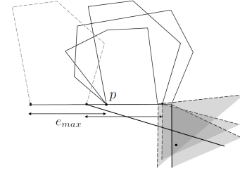
Fig. 8. The intersection of the corresponding regions to all candidate vertices.
