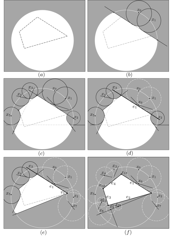
Fig. 1. An illustration of Algorithm 1 probing to determine the shape and location of a polygon with n = 4 vertices and k = 1 acute angle. This instance is solved with 14 ( \leq 3.5n + k + 2 ) probes.
