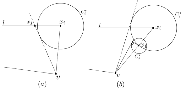
Fig. 5. v is the vertex identified by an undesirable confirmation and C_i^* is the p-disk generated by the subsequent probe. (a) Any probe which falls on l before the next undesirable confirmation of a vertex must be the intersection of l and a line on \partial(R) where the angle at the intersection is not acute, and must be the result of case (b) of Algorithm 1. (b) Any probe after x_i which is the last probe lying on l falls on the intersection of \zeta_i and a tangent line.
